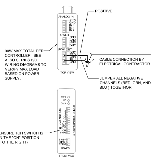
SERIES B/C LIGHTWILD LED LIGHTING CONTROLLER
