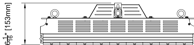
END VIEW
