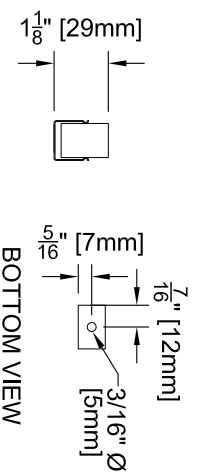
FIXED MOUNTING CLIP
